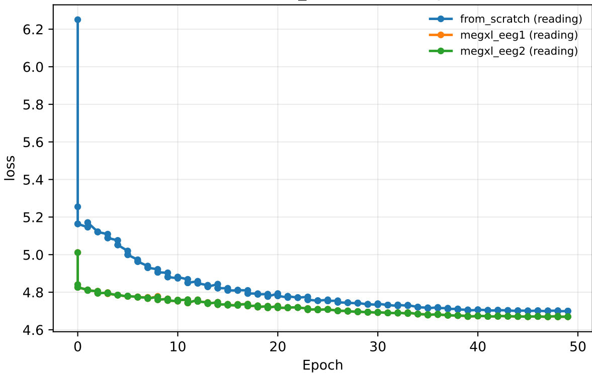
curriculum 20260629_004853 · reading · val/loss
