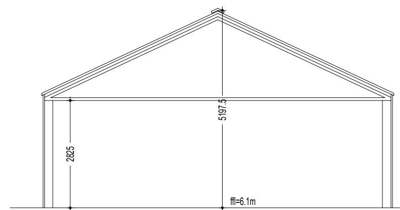
PROPOSED SECTION A - A 1:100
