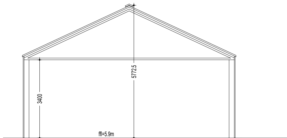
PROPOSED SECTION B - B 1:100
