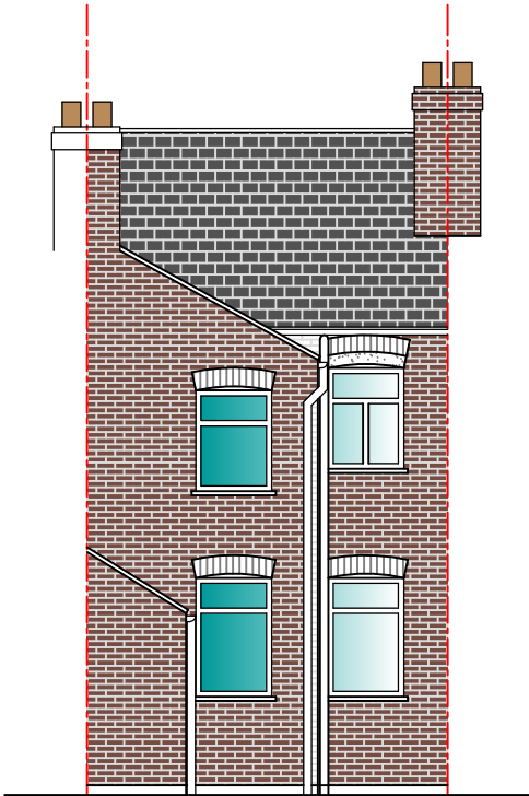
Existing Rear Elevation @ 1:100 (A3)
