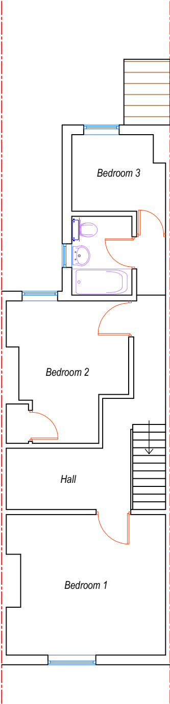
Existing First Floor Plan @ 1:100 (A3)
