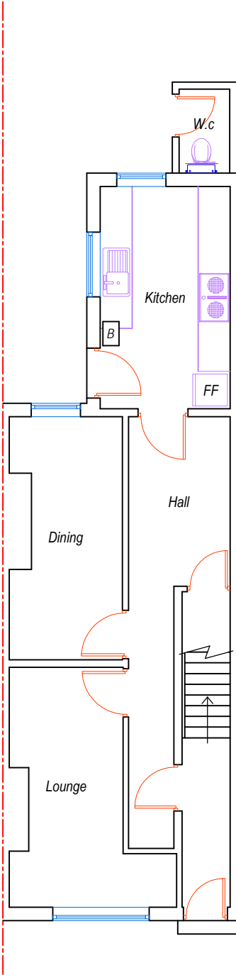
Existing Ground Floor Plan @ 1:100 (A3)
