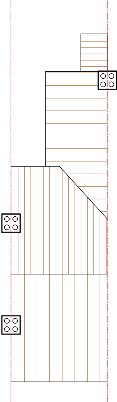
Existing Roof Plan @ 1:100 (A3)
