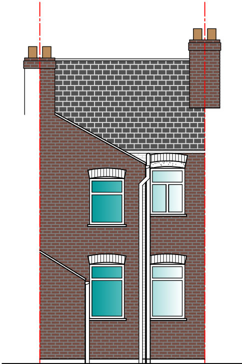
Proposed Rear Elevation @ 1:100 (A3) (UNCHANGED)
