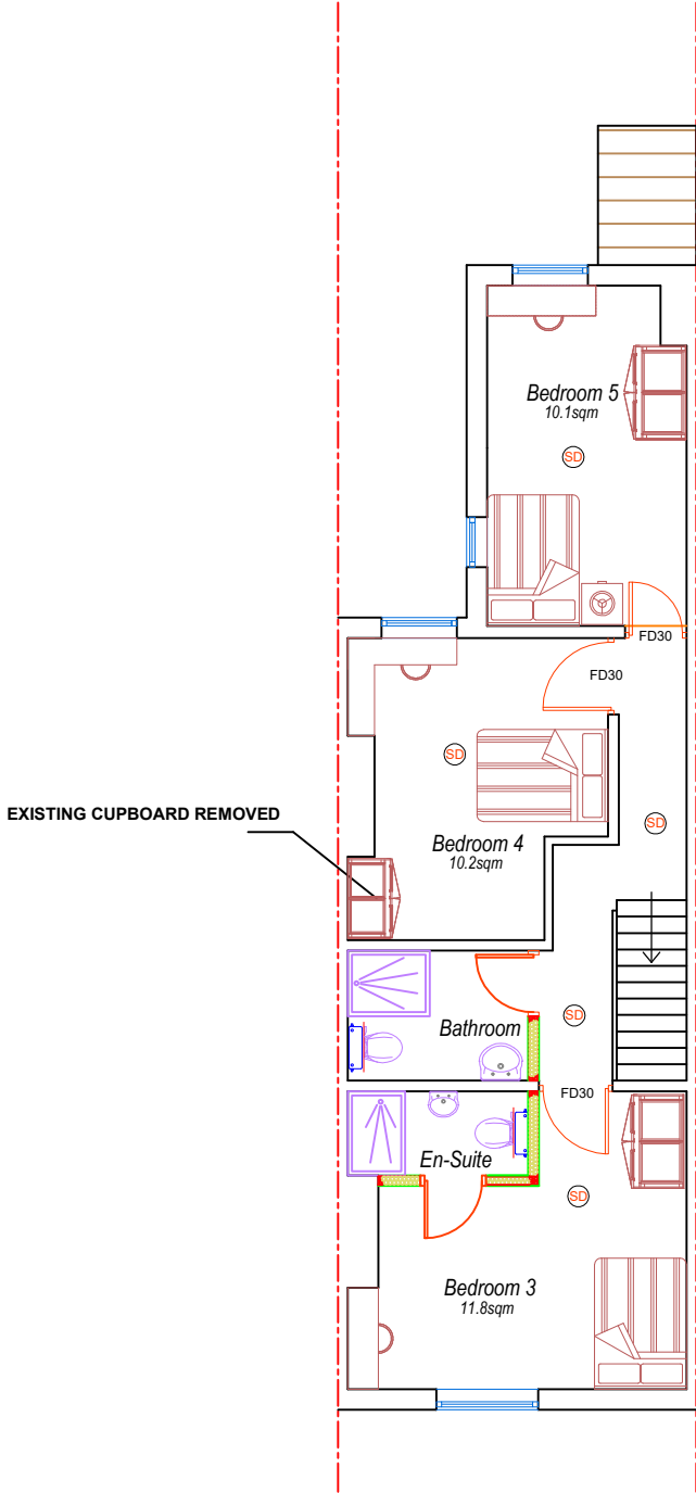
Proposed First Floor Plan @ 1:100 (A3)
