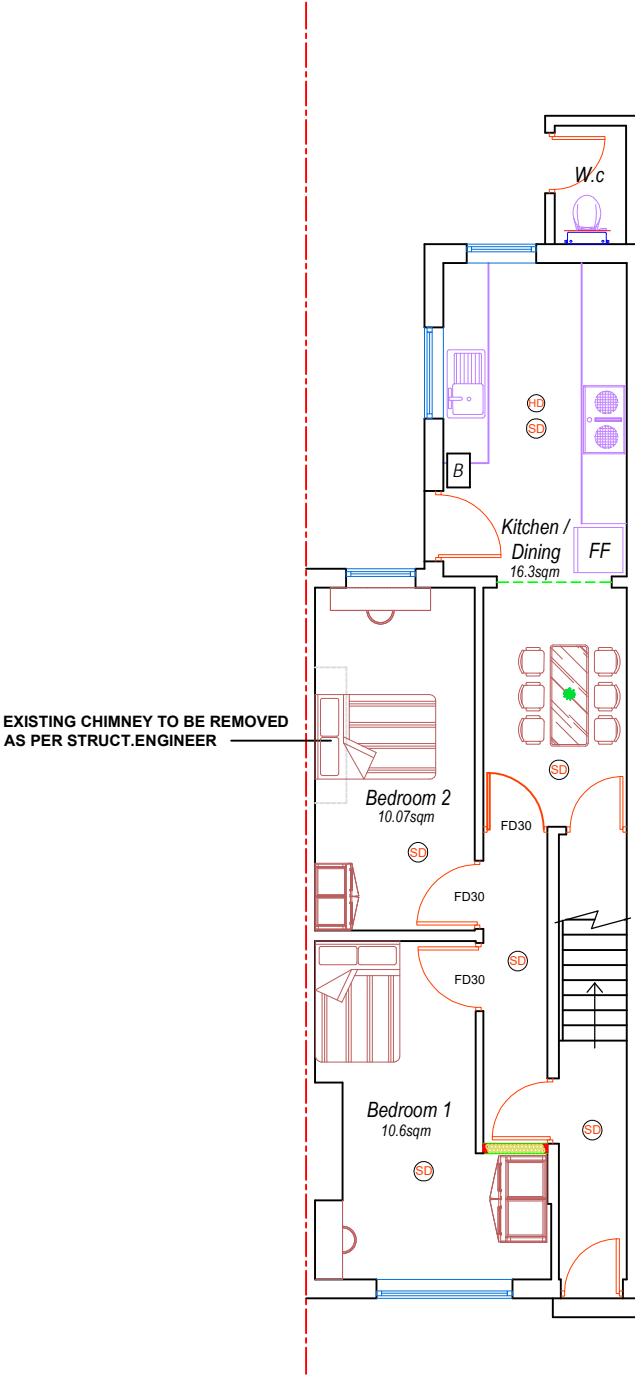
Proposed Ground Floor Plan @ 1:100 (A3)
