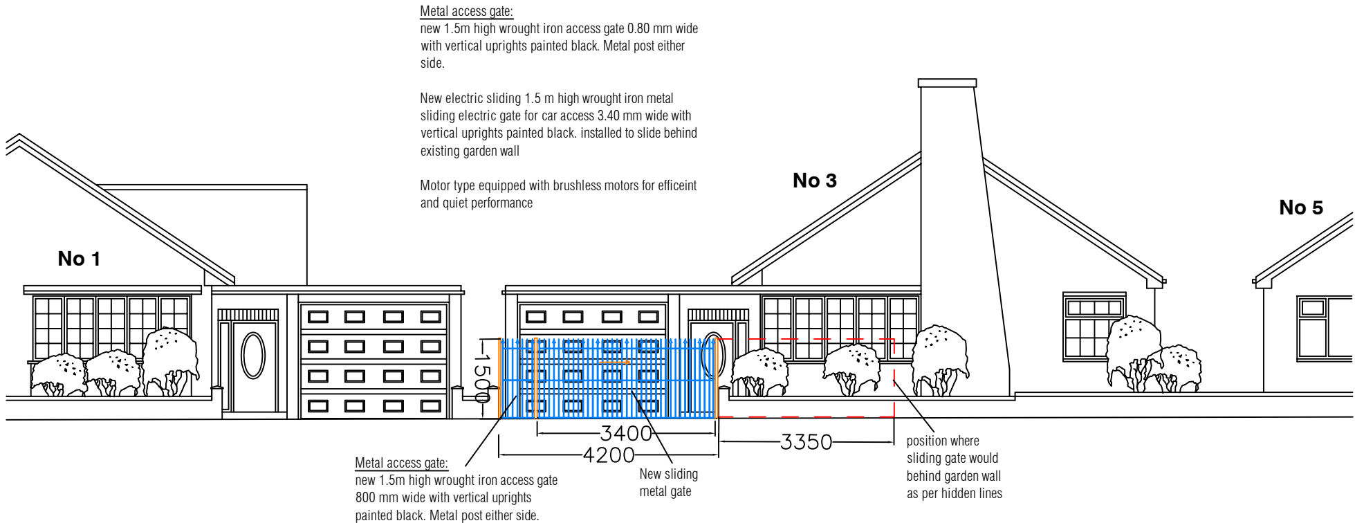
PROPOSED FRONT ELEVATION (FROM STREET), 1:100
