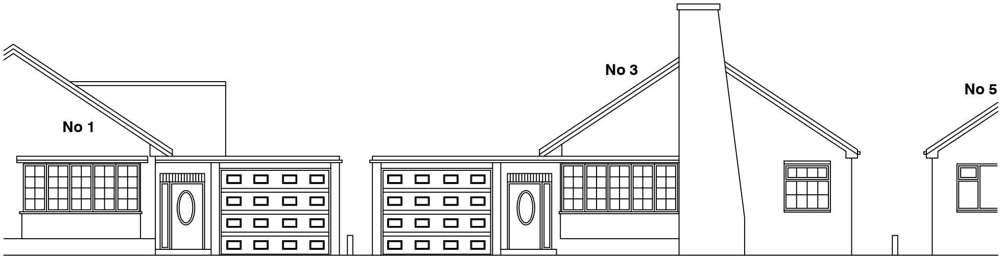
PROPOSED FRONT ELEVATION (FROM GARDEN), 1:100
