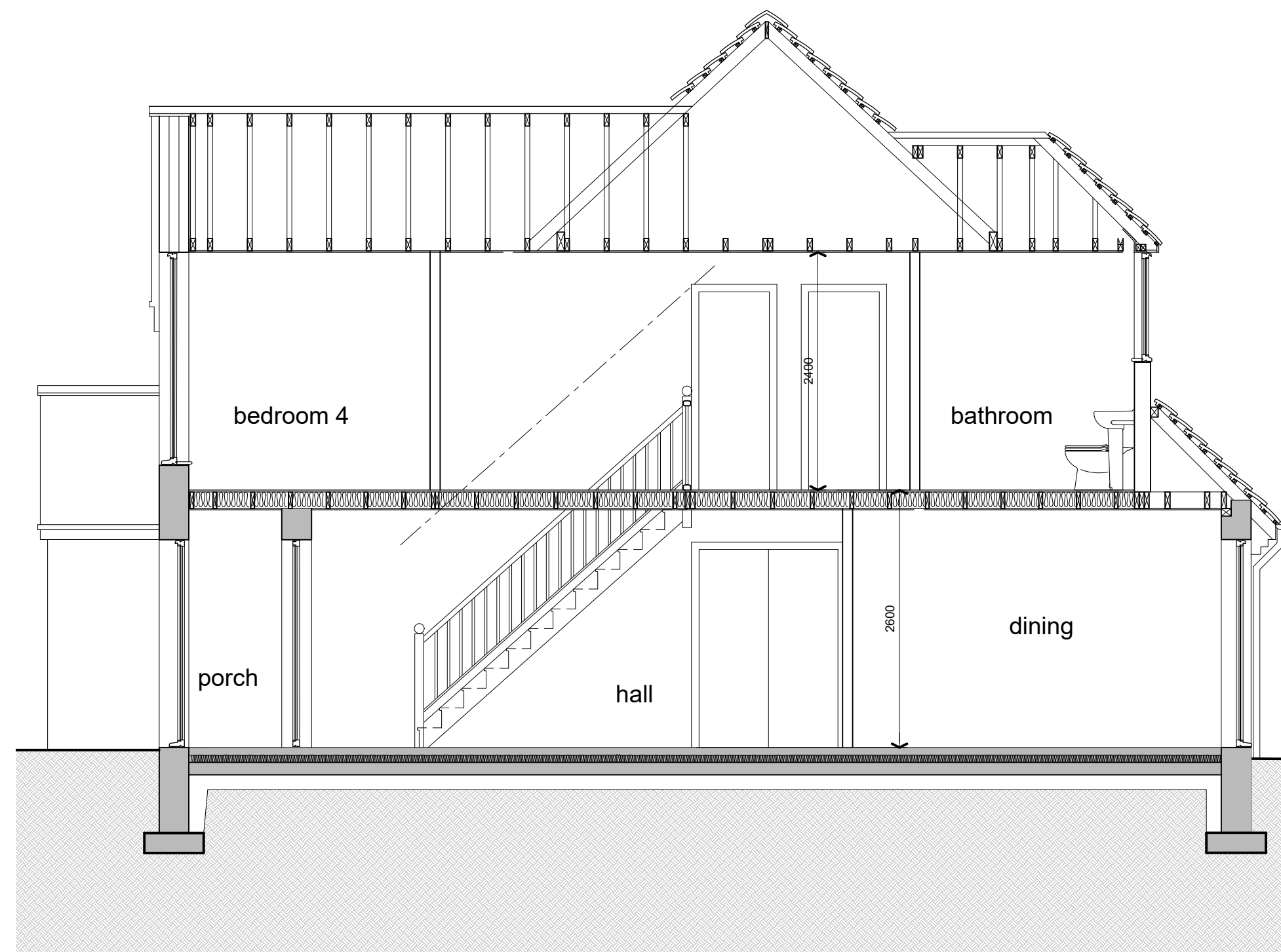
a proposed section Scale: 1:50
