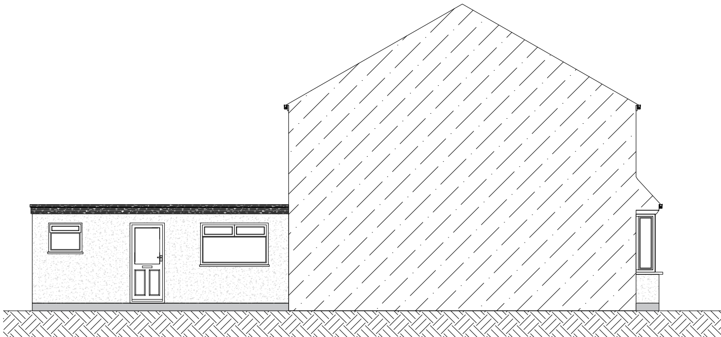
SIDE ELEVATION (Party wall)
