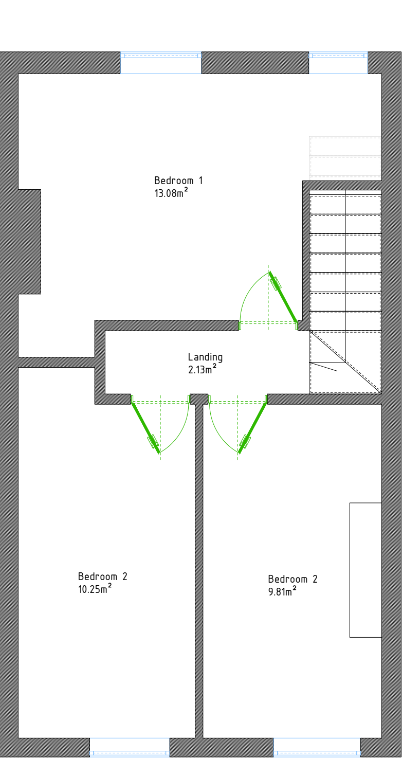
EXISTING FIRST FLOOR PLAN 1:50@A2
