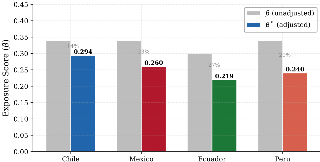
Figure X: Technical vs. Adjusted LLM Exposure Scores
