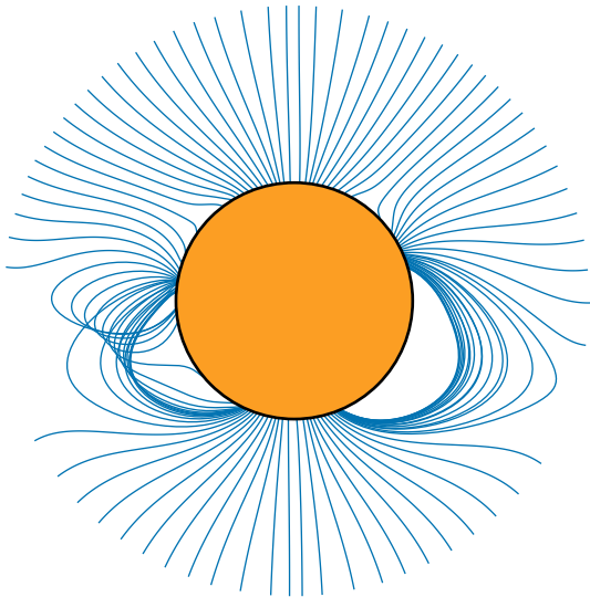
Outflow, r_{ss} = 2.5R_{\odot}
