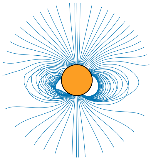
Outflow, r_{ss} = 5.0R_{\odot}
