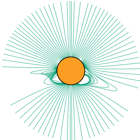
Outflow, r_{ss} = 5.0R_{\odot}
