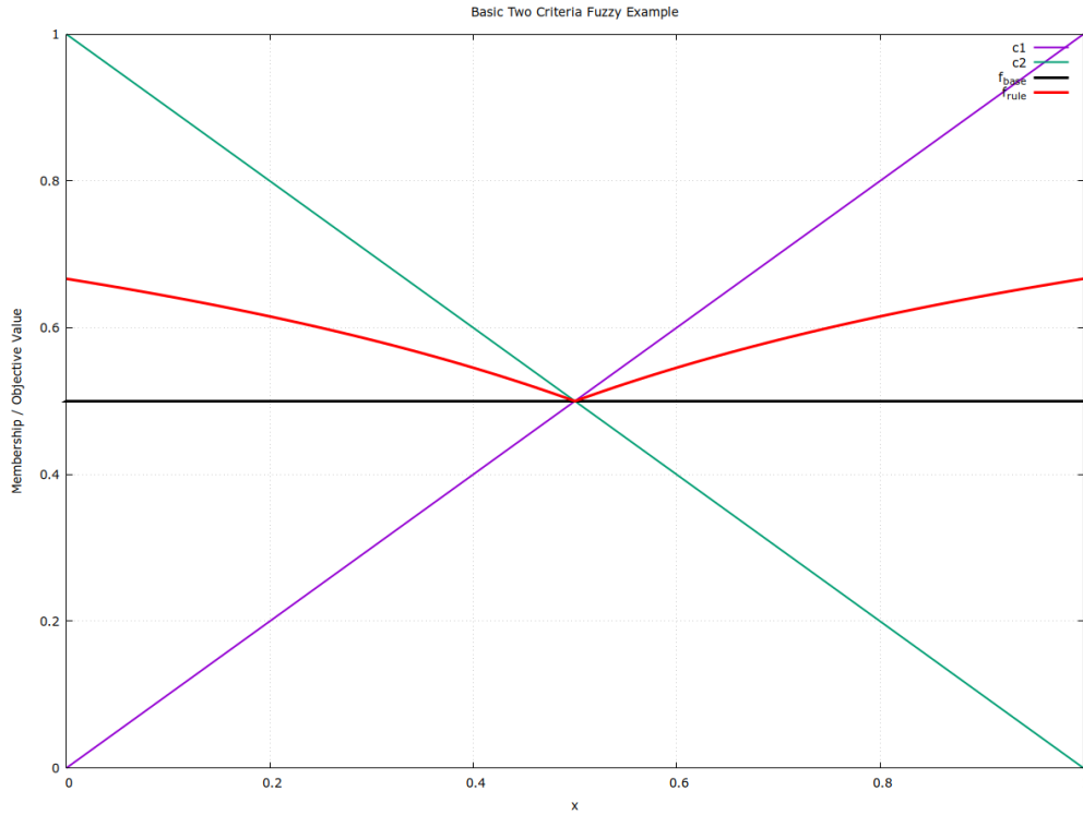
Figure 1: Output of the first example. The plot compares the two criteria c_1 = x and c_2 = 1 - x , the base objective f_{\text{base}} , and the rule-based objective f_{\text{rule}} . Without the explicit rule, the two opposing criteria balance each other exactly, resulting in the constant neutral value f_{\text{base}} = 0.5 . The additional rule penalizes undesirable extreme solutions and therefore changes the shape of the objective.
