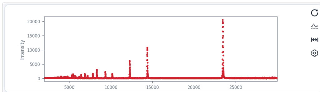
Figure 8: The raw data file for a pattern that has never been refined yet.
