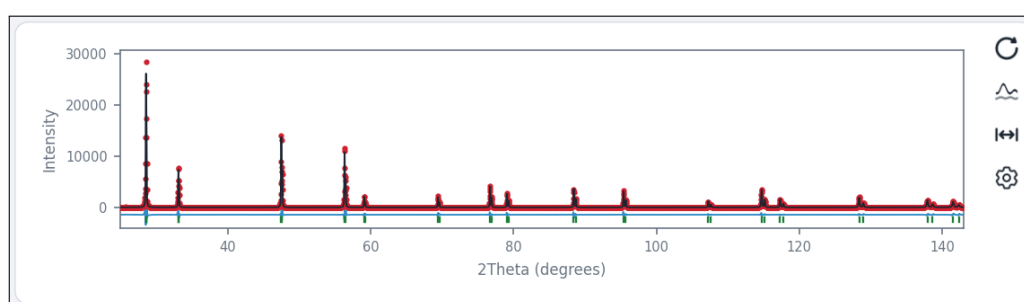
Figure 9: The same panel once a .prf exists: observed points, the calculated curve, the difference below it, and reflection positions as tick marks.
