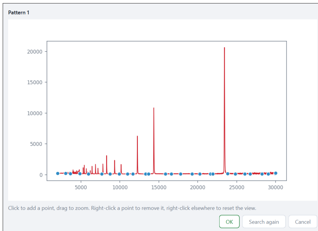
Figure 10: Determine background... , already seeded with an automatic search (blue points) over raw TOF data.
