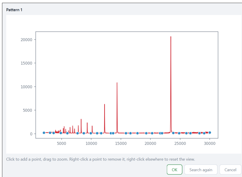
Figure 9: Determine background... , already seeded with an automatic search (blue points) over raw TOF data.
