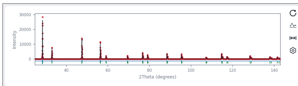
Figure 8: The same panel once a .prf exists: observed points, the calculated curve, the difference below it, and reflection positions as tick marks.
