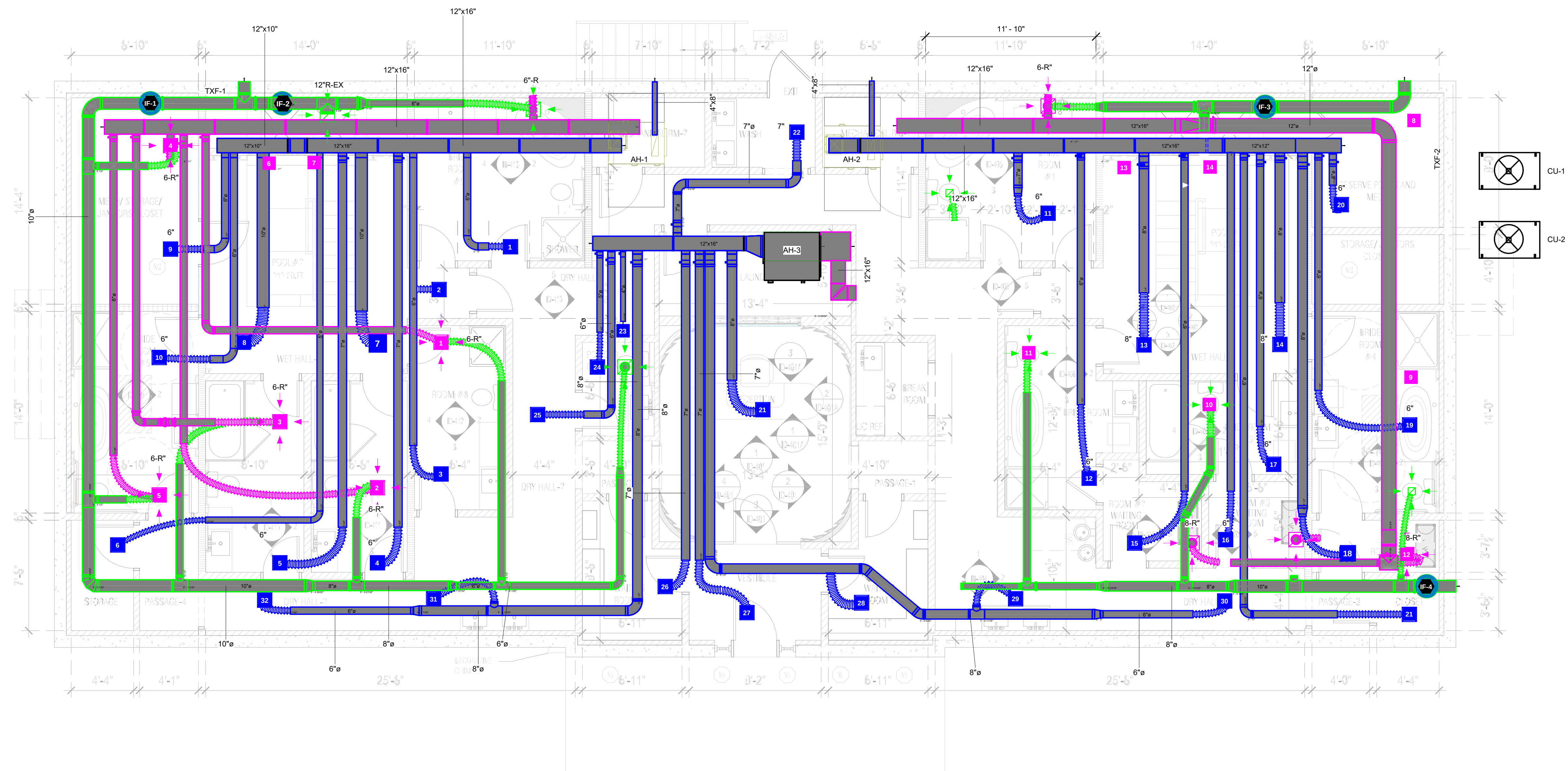
1 FIRST FLOOR LAYOUT SCALE: 1/8" = 1'-0"
