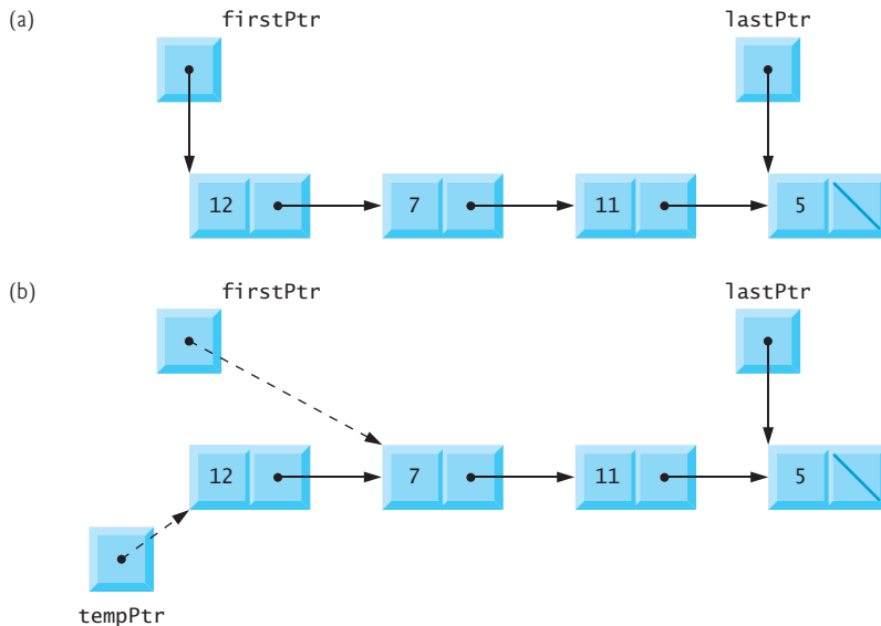
Fig. 19.8 | Operation removeFromFront represented graphically.
