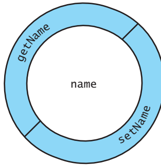
Fig. 3.7 | Conceptual view of an Account object with its encapsulated private data member name and protective layer of public member functions.
