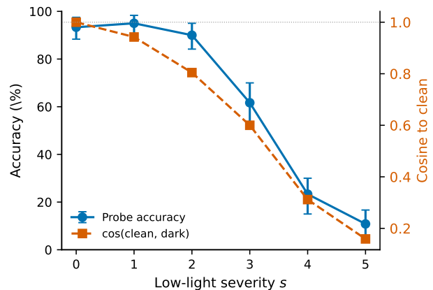
Figure 1. Accuracy (blue, left axis; error bars 95% CI) and mean cosine similarity to clean embeddings (red, right axis) vs. severity. The two curves dissociate: drift is smooth, the decision is not. Accuracy at severity 1 never falls below clean across nine seed \times regularization configurations (§9).
