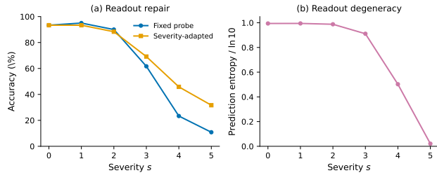
Figure 3. (a) Fixed vs. severity-adapted probe accuracy. (b) Prediction entropy (normalized by \ln 10 ): the fixed readout degenerates toward a constant class as severity grows.
