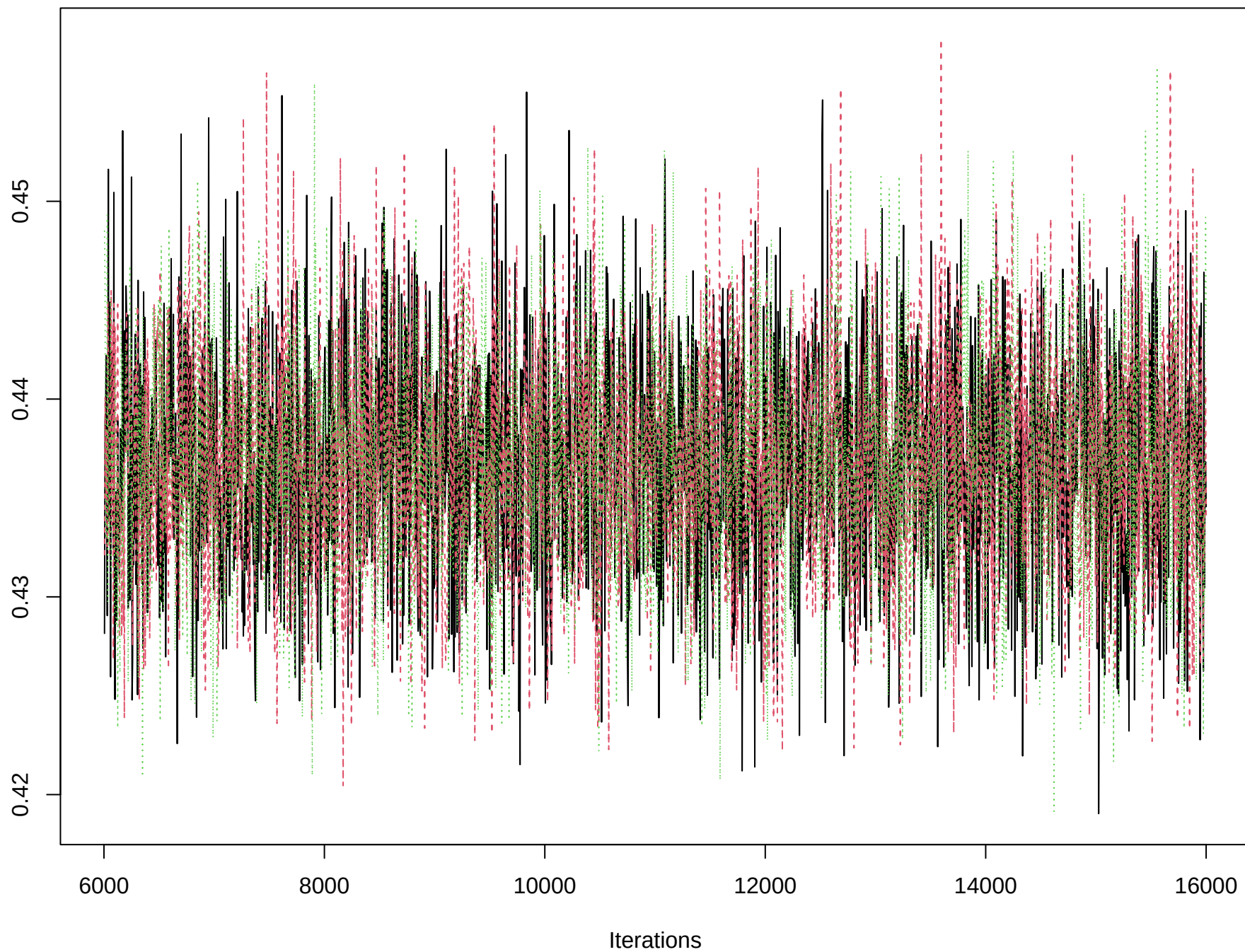
Trace of sigma
