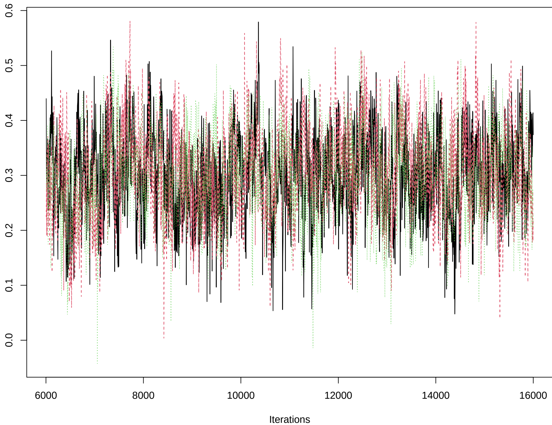
Trace of \mu_\alpha
