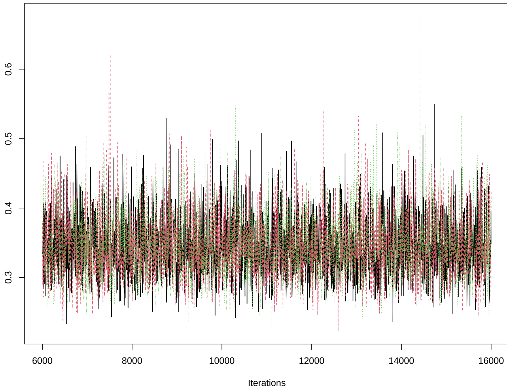
Trace of sigma_alpha
