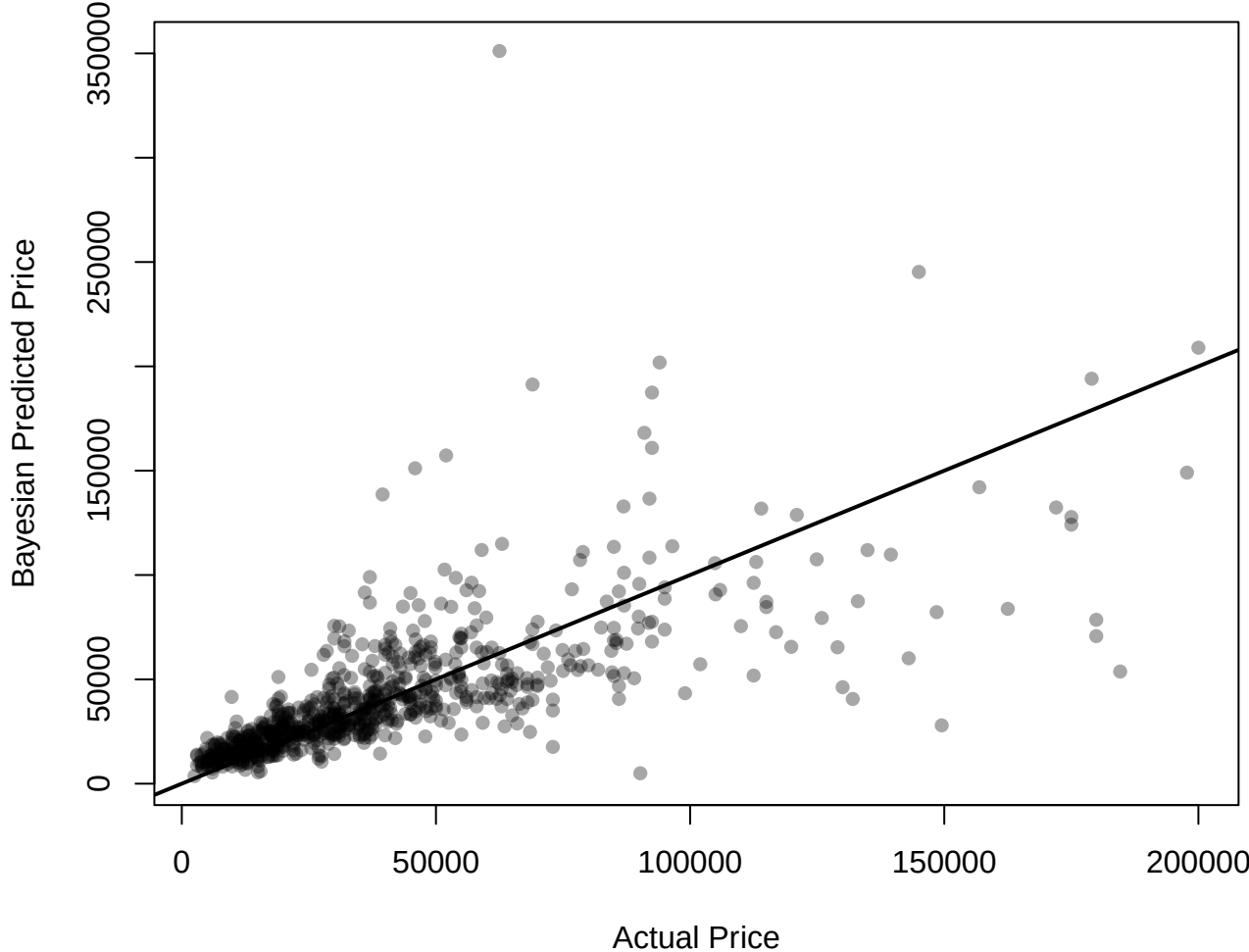
Actual vs Predicted Used Car Prices: Bayesian Hierarchical Model
