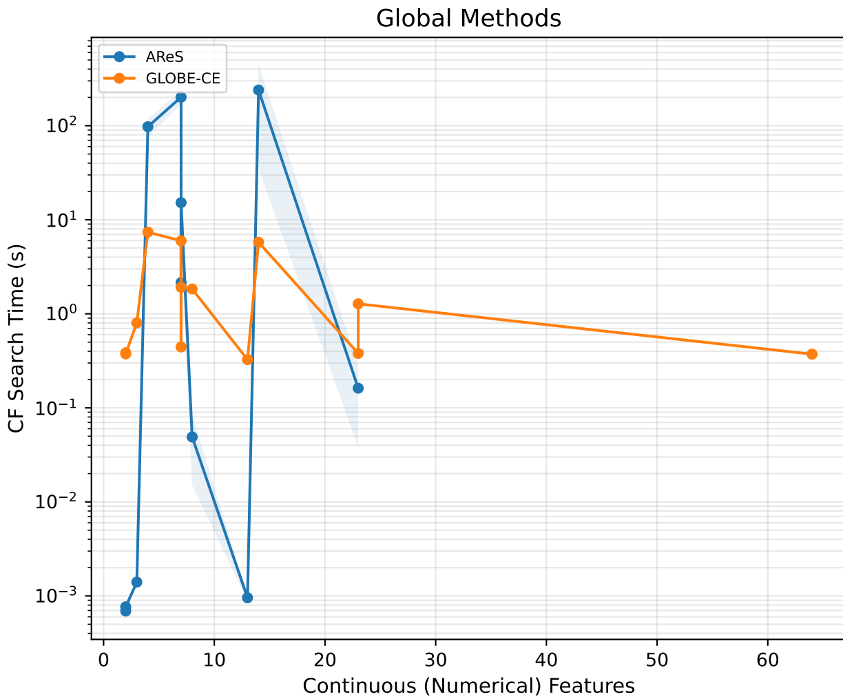
CF Search Time Scaling — Continuous vs. Total Features (MLPClassifier)
