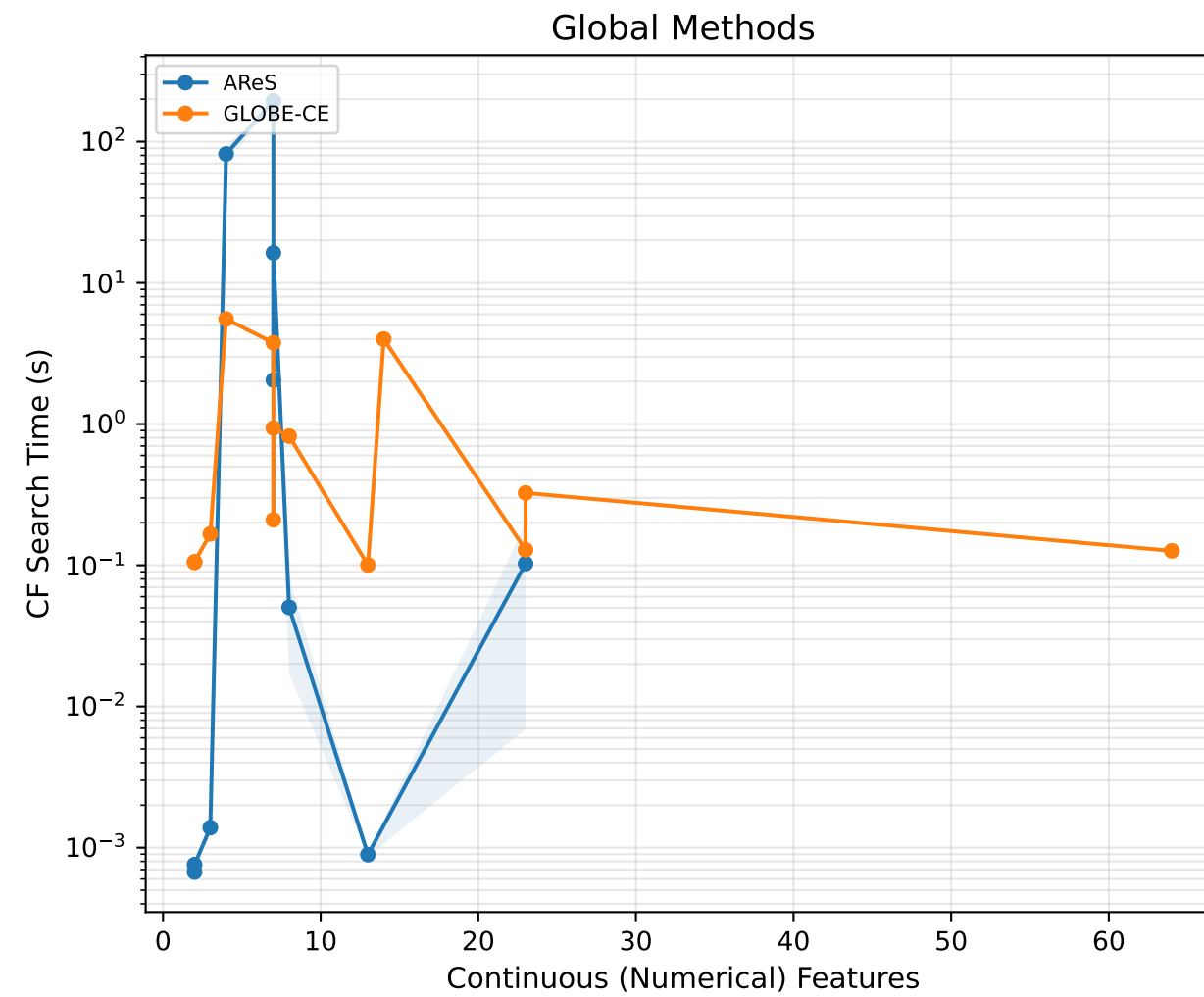
CF Search Time Scaling — Continuous vs. Total Features (MultinomialLogisticRegression)
