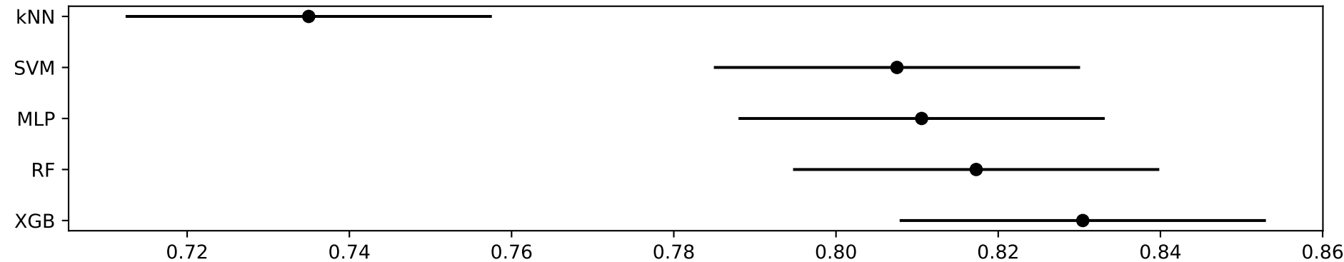
Confidence Interval Plot - Model Comparison ( \alpha = 0.05 )
