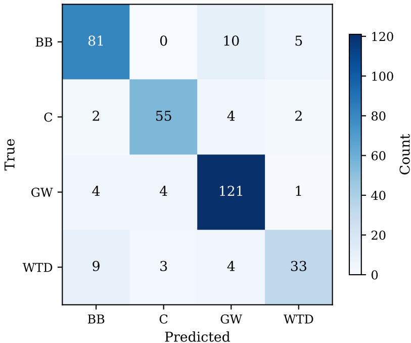
Confusion Matrix (k=17)
