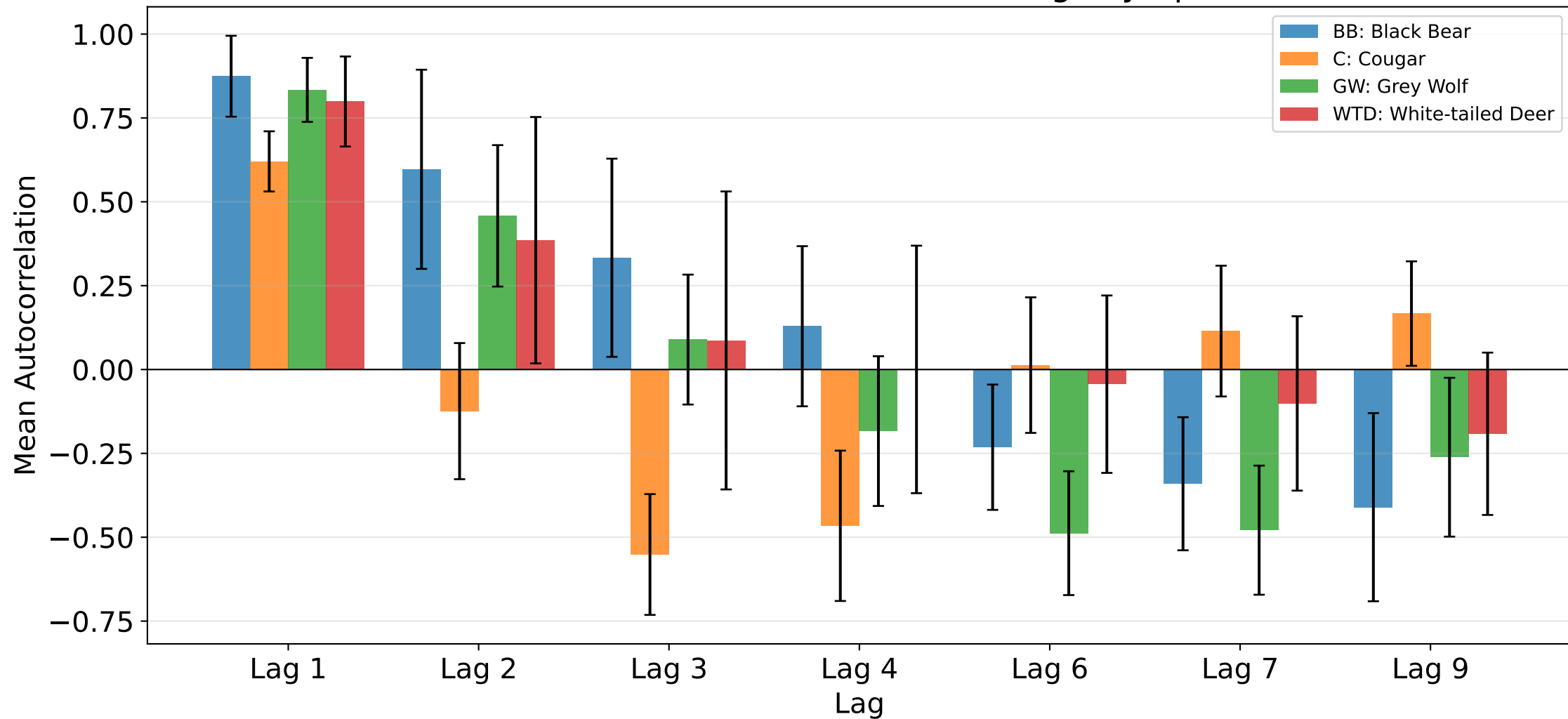
Mean Autocorrelation at Selected Lags by Species
