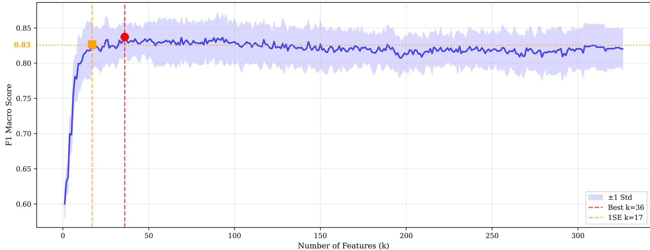
RFE Feature Elimination Path
