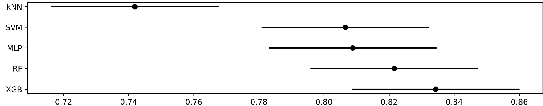
Confidence Interval Plot — Extended Features ( \alpha = 0.05 )
