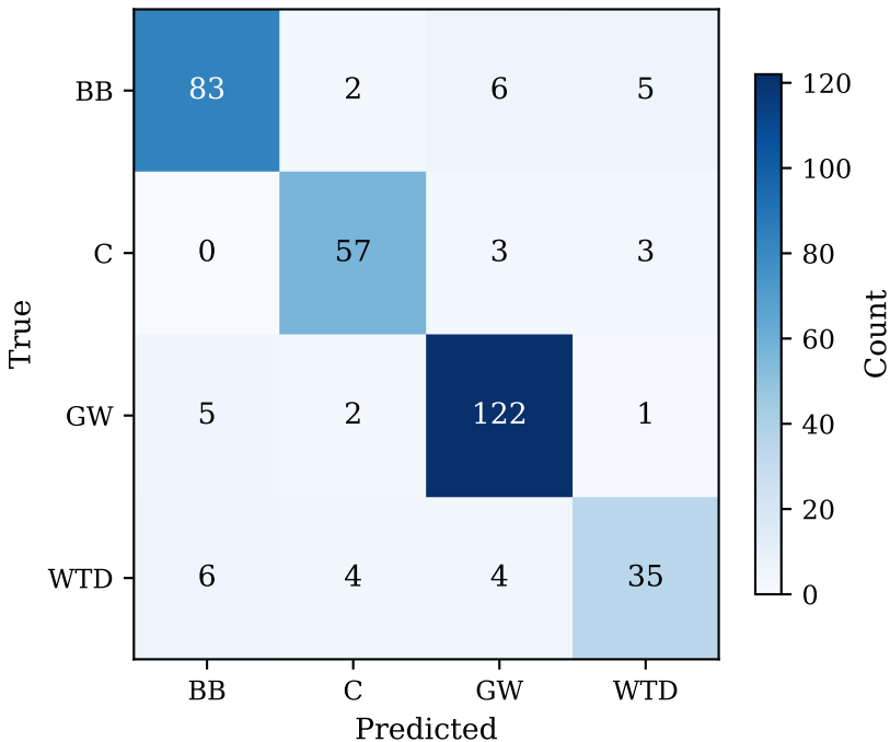
Confusion Matrix (k=24)
