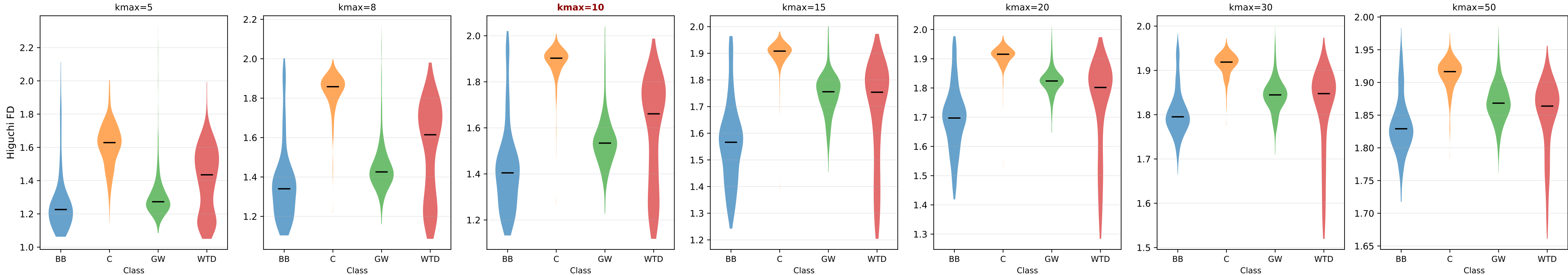
Higuchi FD Distributions by Class at Different kmax Values (kmax=10 in red = value used in exp002)
