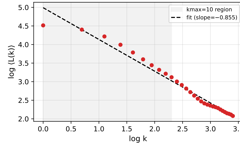
WTD: White-tailed Deer HFD \approx 0.855
