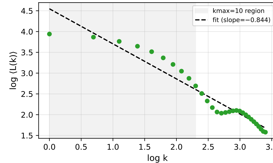
GW: Grey Wolf HFD \approx 0.844
