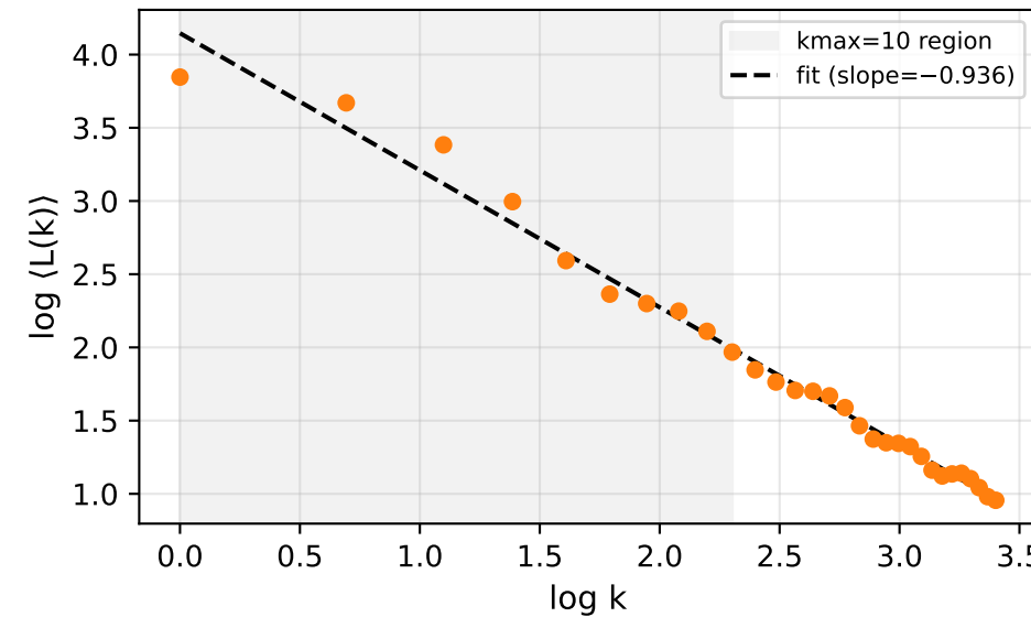
C: Cougar HFD \approx 0.936
