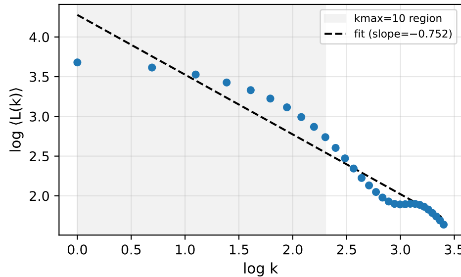
BB: Black Bear HFD \approx 0.752
