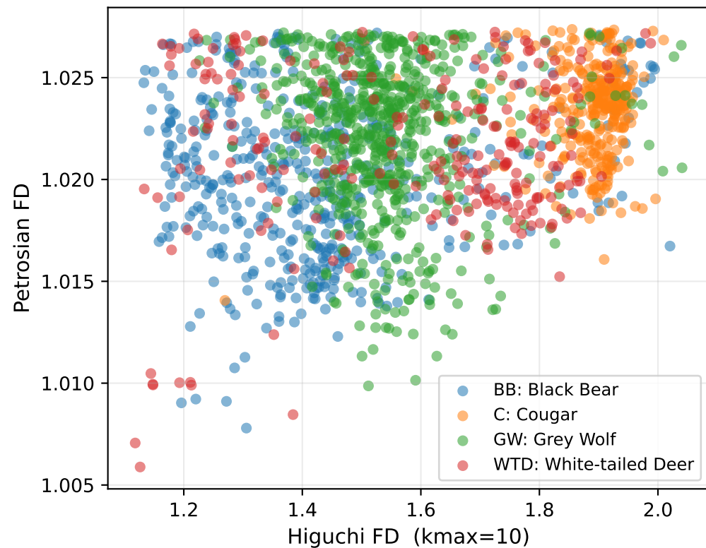
HFD vs PFD — Relationship Between Both Fractal Measures
