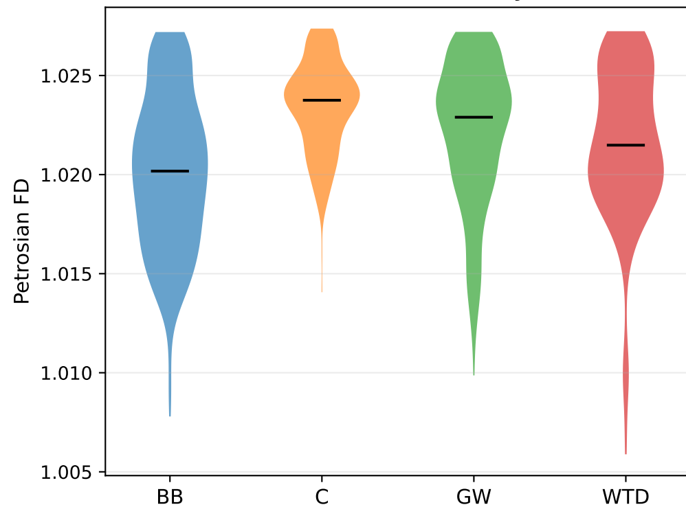
Petrosian FD Distribution by Class
