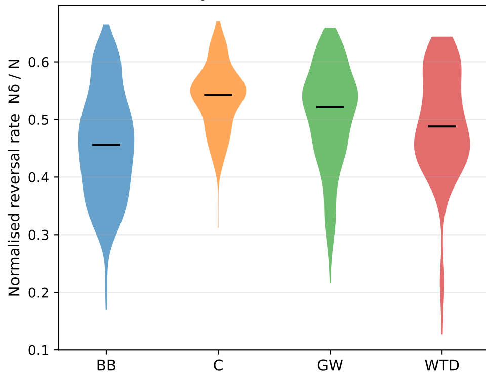
Sign-Reversal Rate by Class (input to Petrosian FD)
