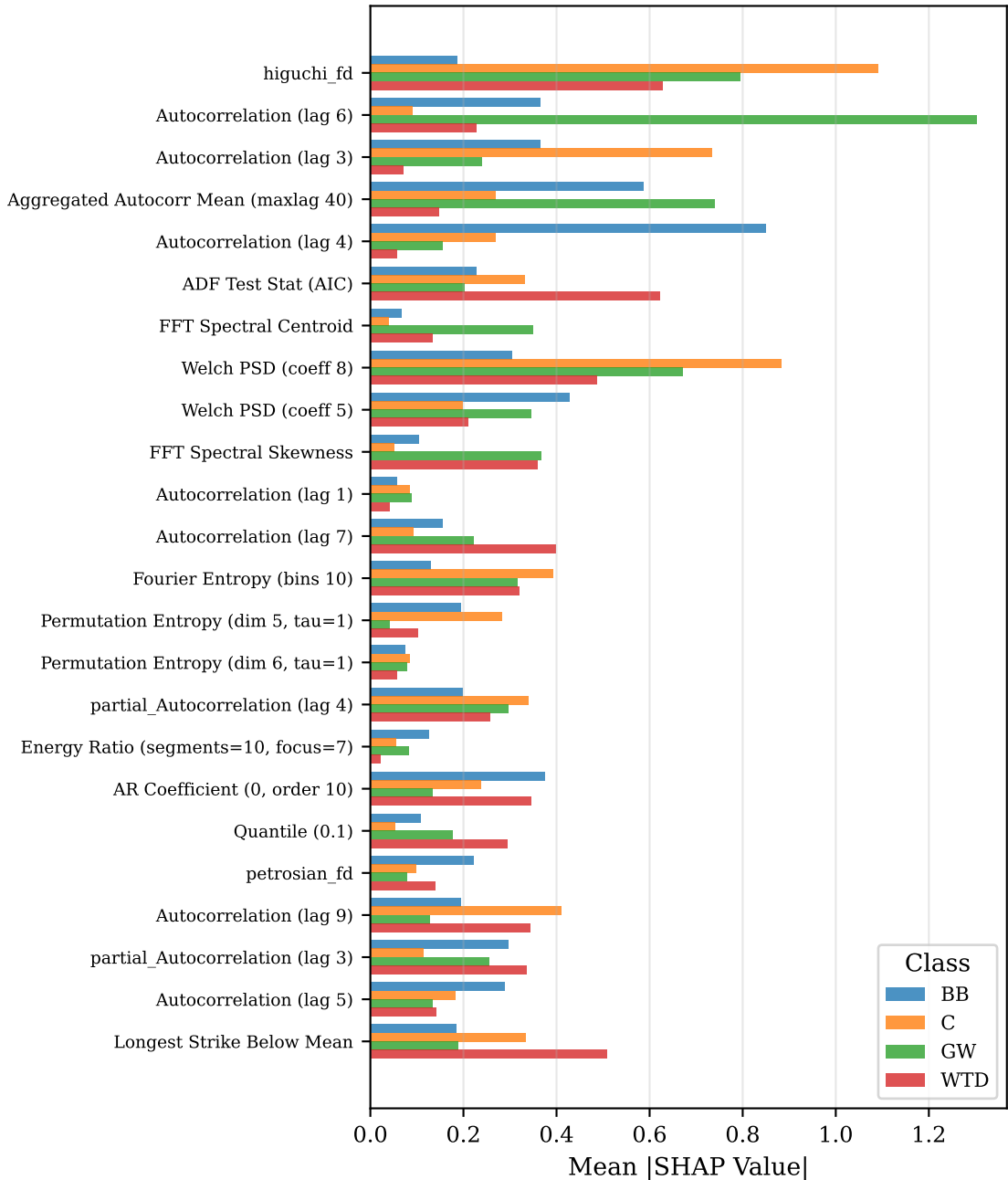
SHAP Feature Importance by Class
