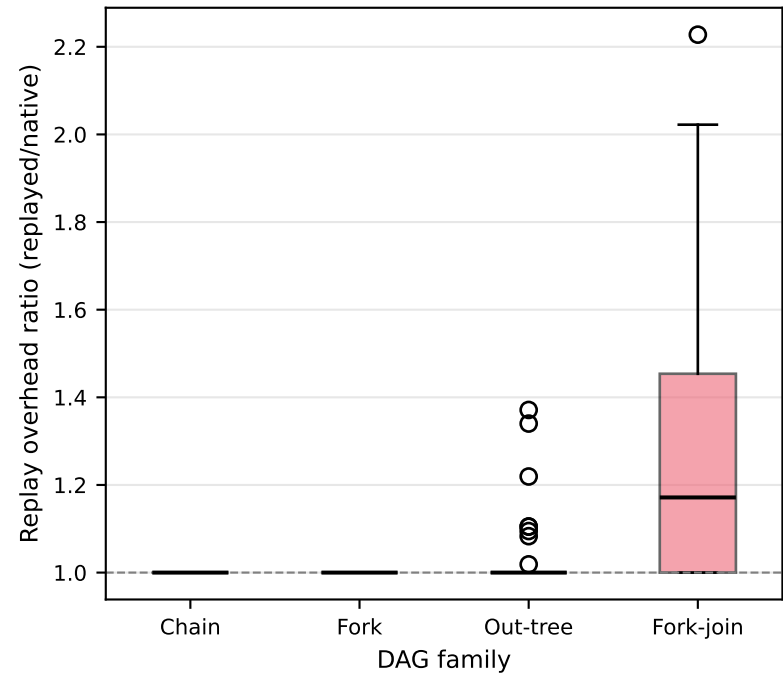
Fig B — Native-model optimism: replay overhead ratio (all CCR, 20 seeds)
