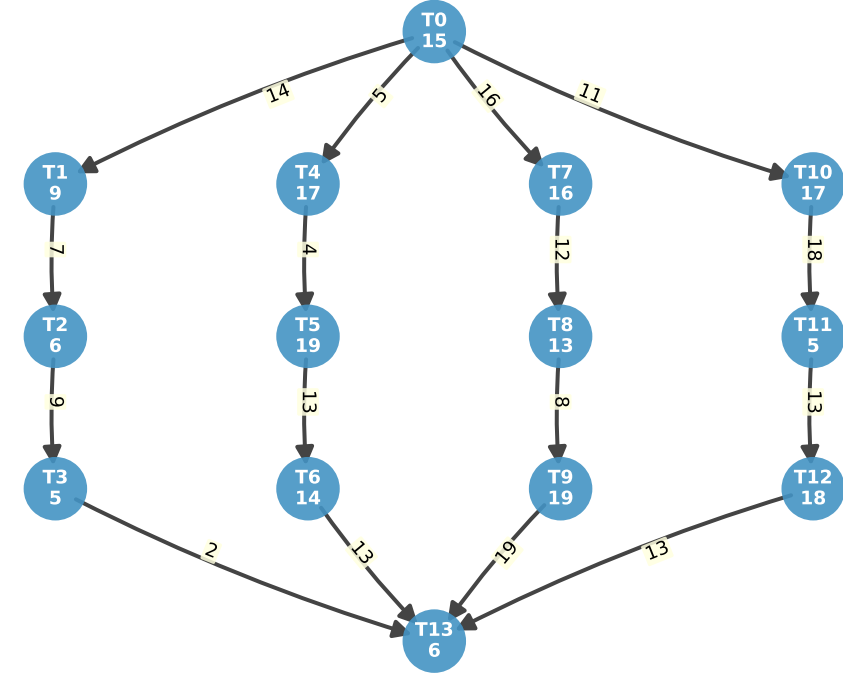
Fork-join 14 tasks, 16 edges, CCR=1.00
