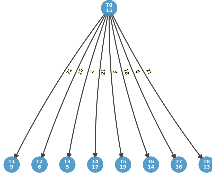
Fork 9 tasks, 8 edges, CCR=1.00
