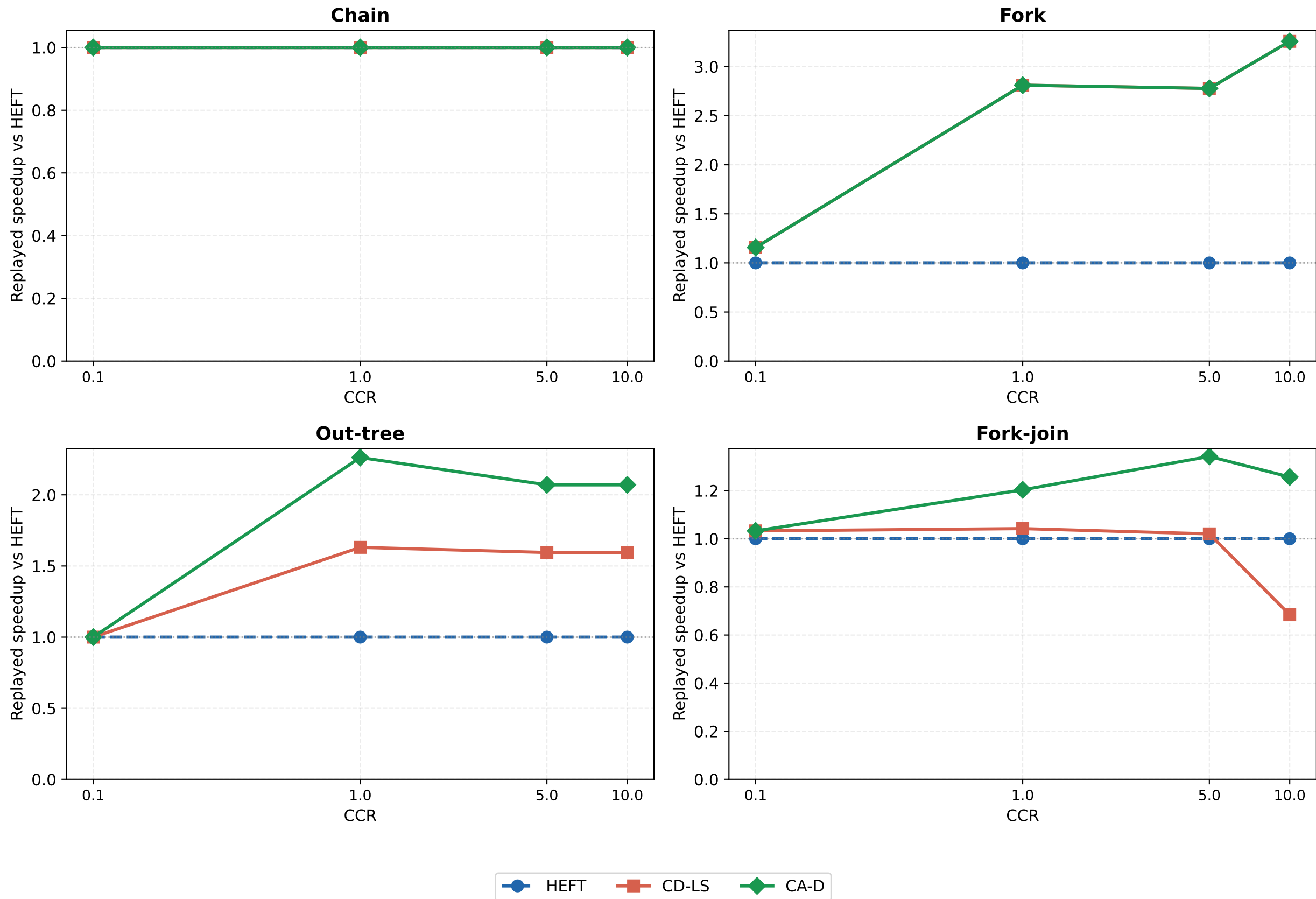
Fig 5 -- CCR sweep: Replayed speedup vs HEFT (seed=0)
