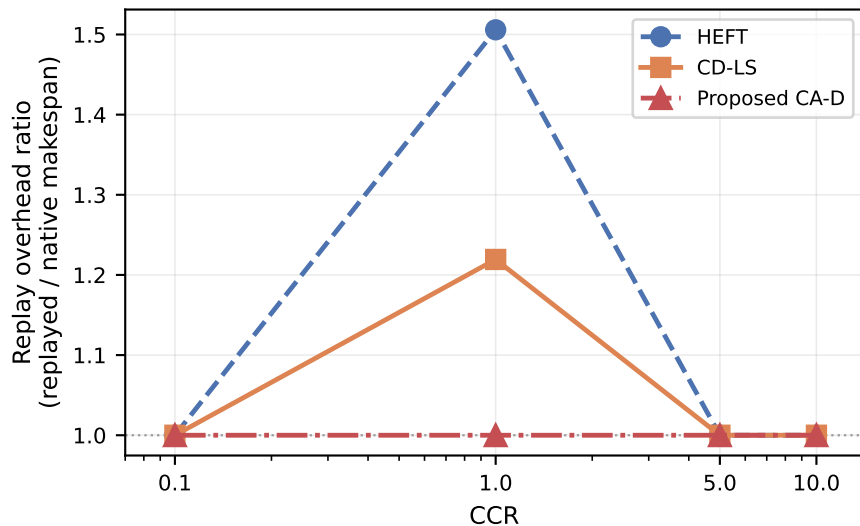
Out-tree
