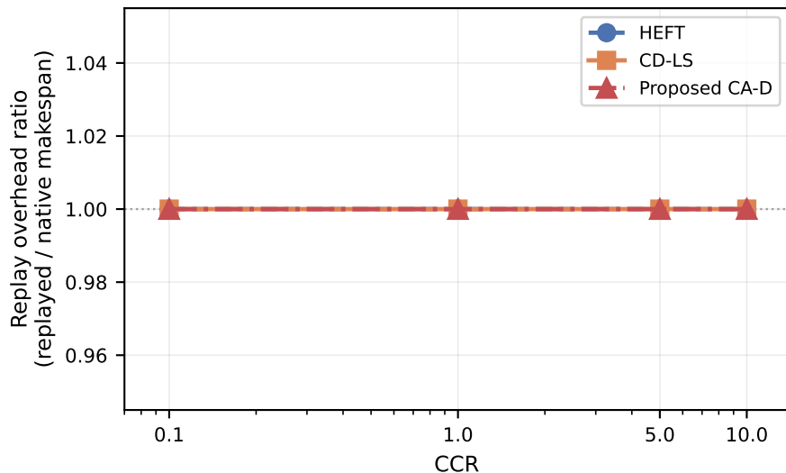
Out-tree
