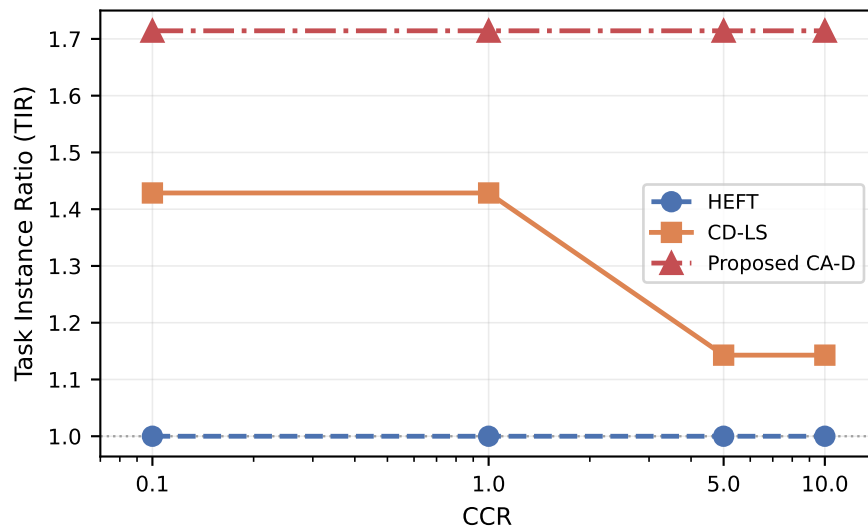
Out-tree
