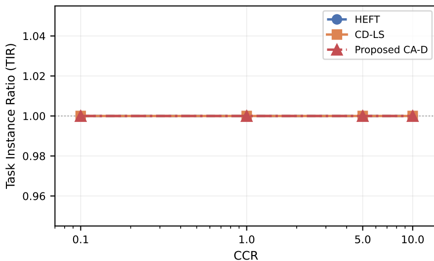
Out-tree
