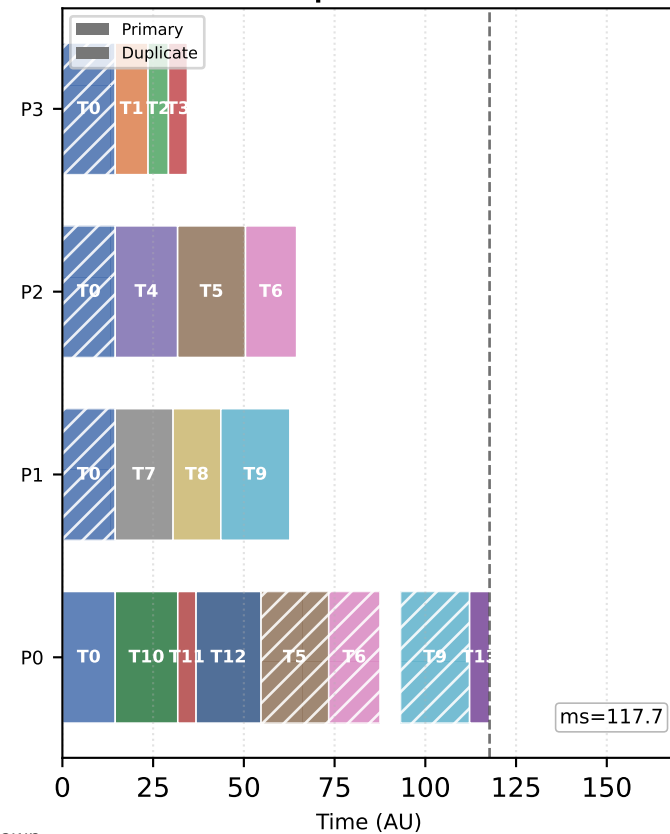
Proposed CA-D
