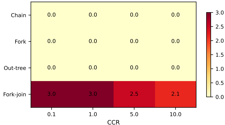
CA-D Mean n_used_links
