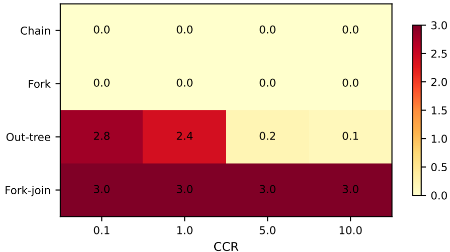
CD-LS Mean n_used_links
