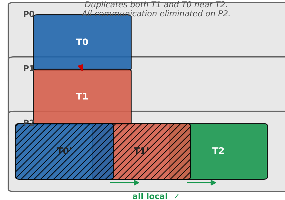
C — CA-D (recursive duplication)
