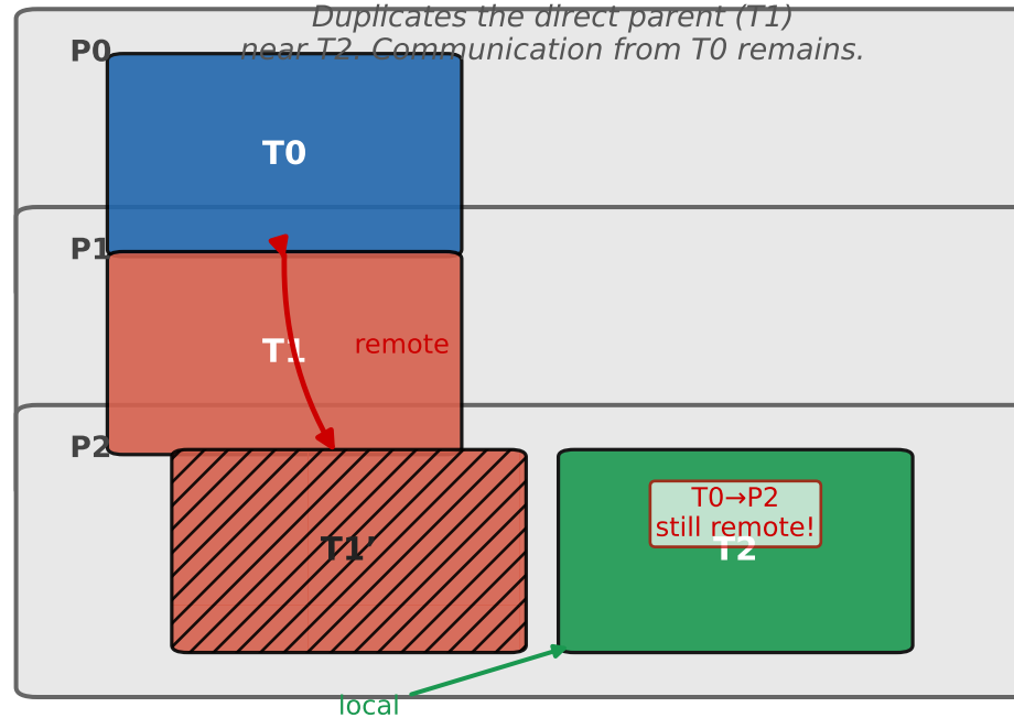
B — CD-LS (parent duplication)
