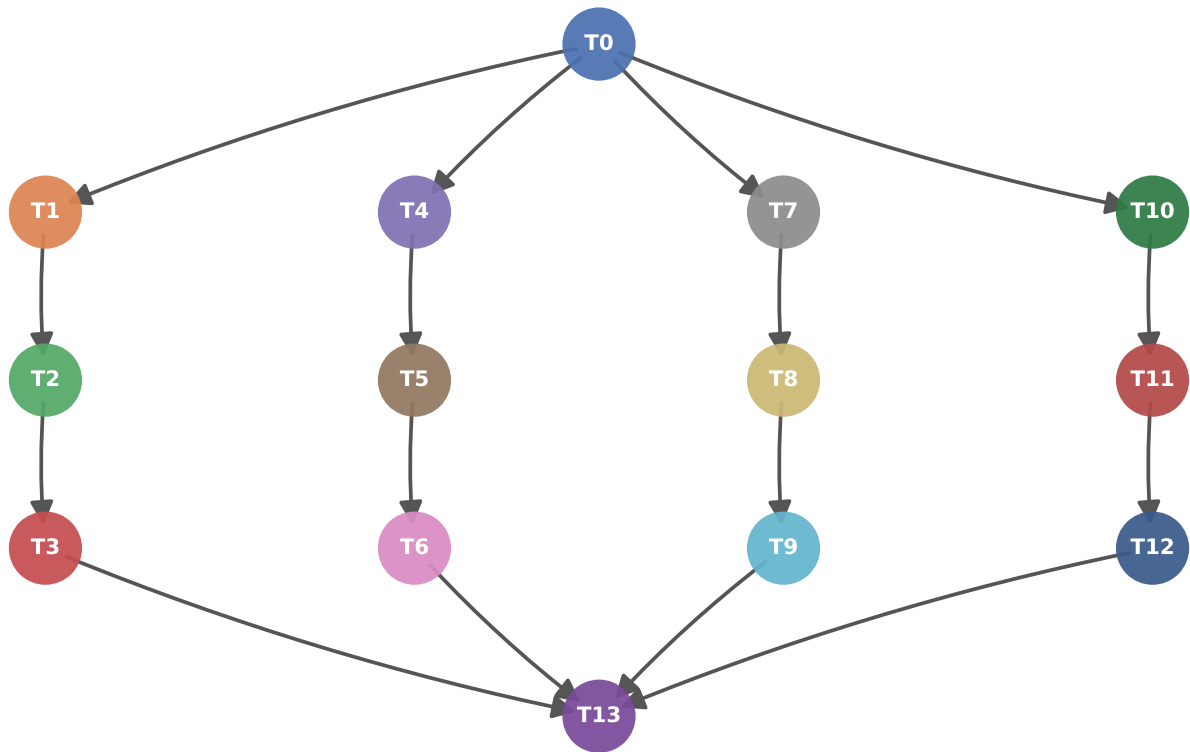
Fork-join DAG topology (n_branches=4, bl=3, CCR=5.0, seed=0)
