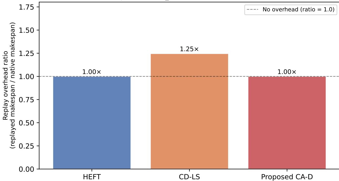
Replay Overhead Ratio Fork-join DAG, n_branches=4, bl=3, CCR=5.0
