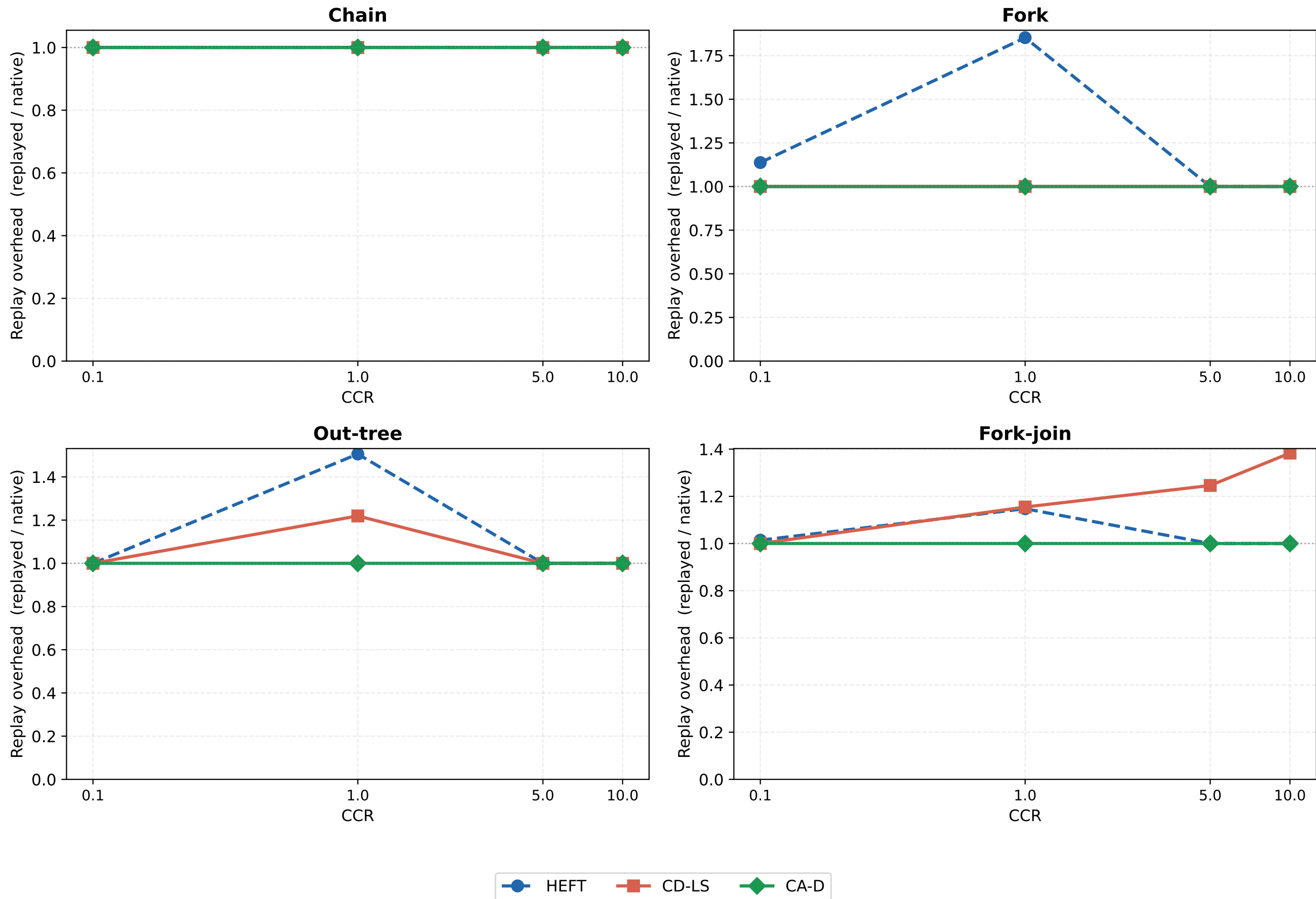
Fig 6 -- CCR sweep: Replay overhead ratio (seed=0)
