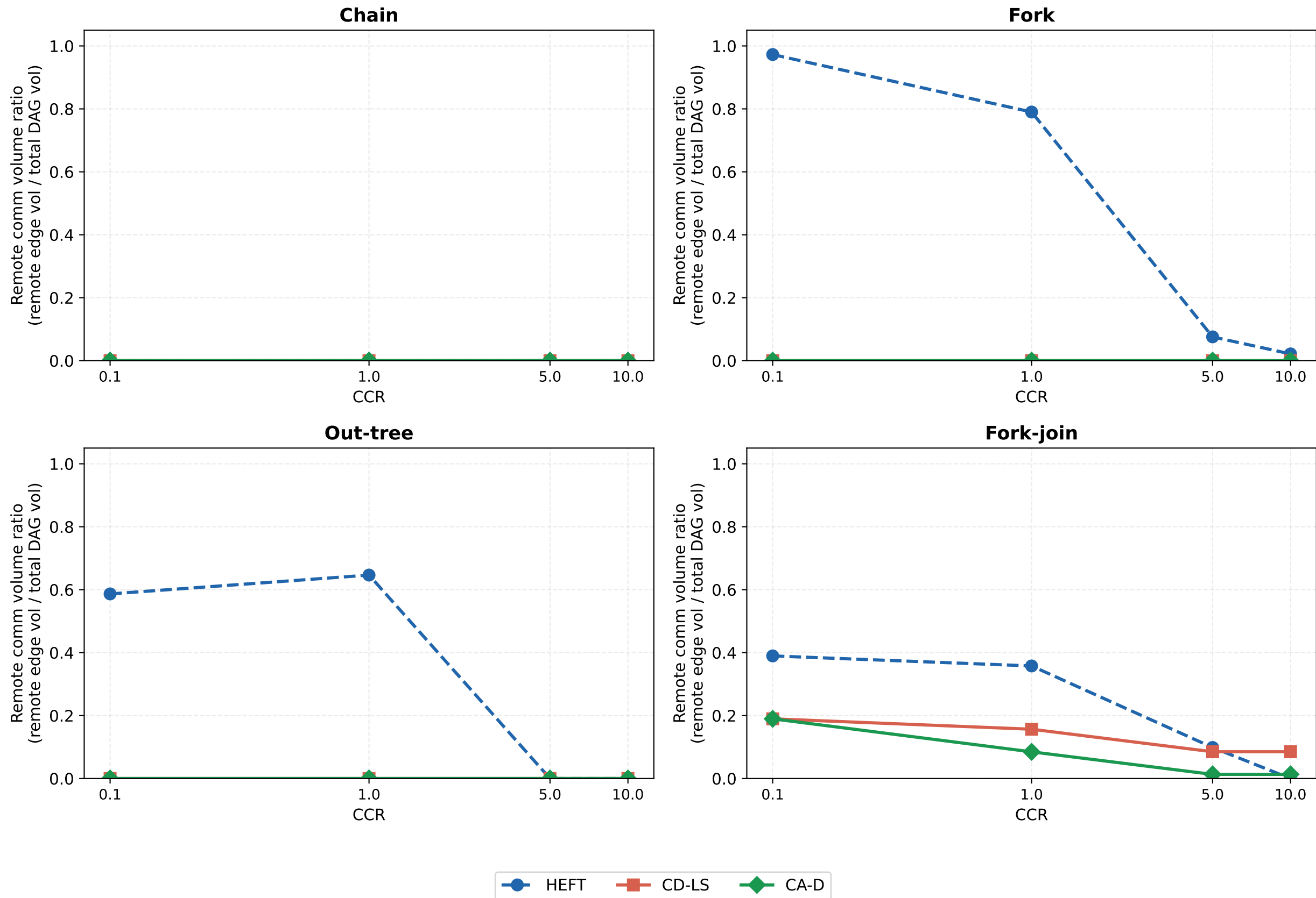
Fig 8 -- CCR sweep: Remote communication volume ratio (seed=0)
