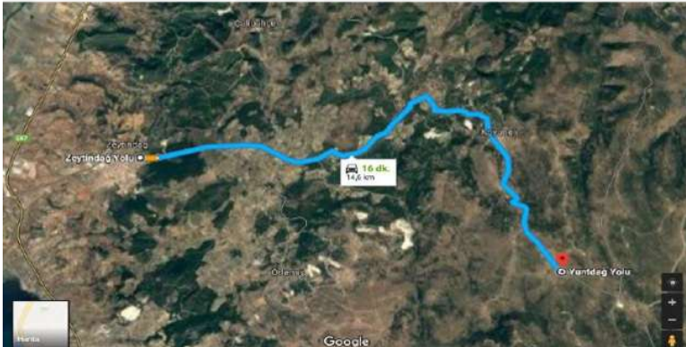
Figure 1. Route engineering study identifying the transportation corridor between the blade storage area and the wind farm site. The survey was undertaken to assess horizontal curves, road widths and geometric constraints to determine the required transportation method.
