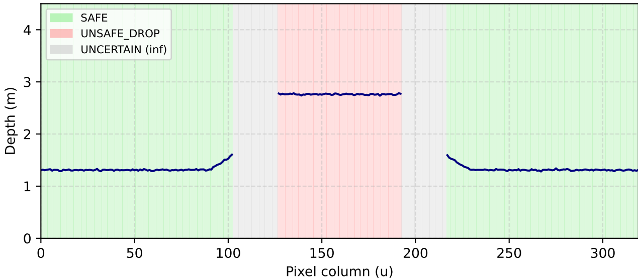
Depth Profile at Row y=120 — Pit Scene Green: SAFE, Red: UNSAFE_DROP, Grey: UNCERTAIN
