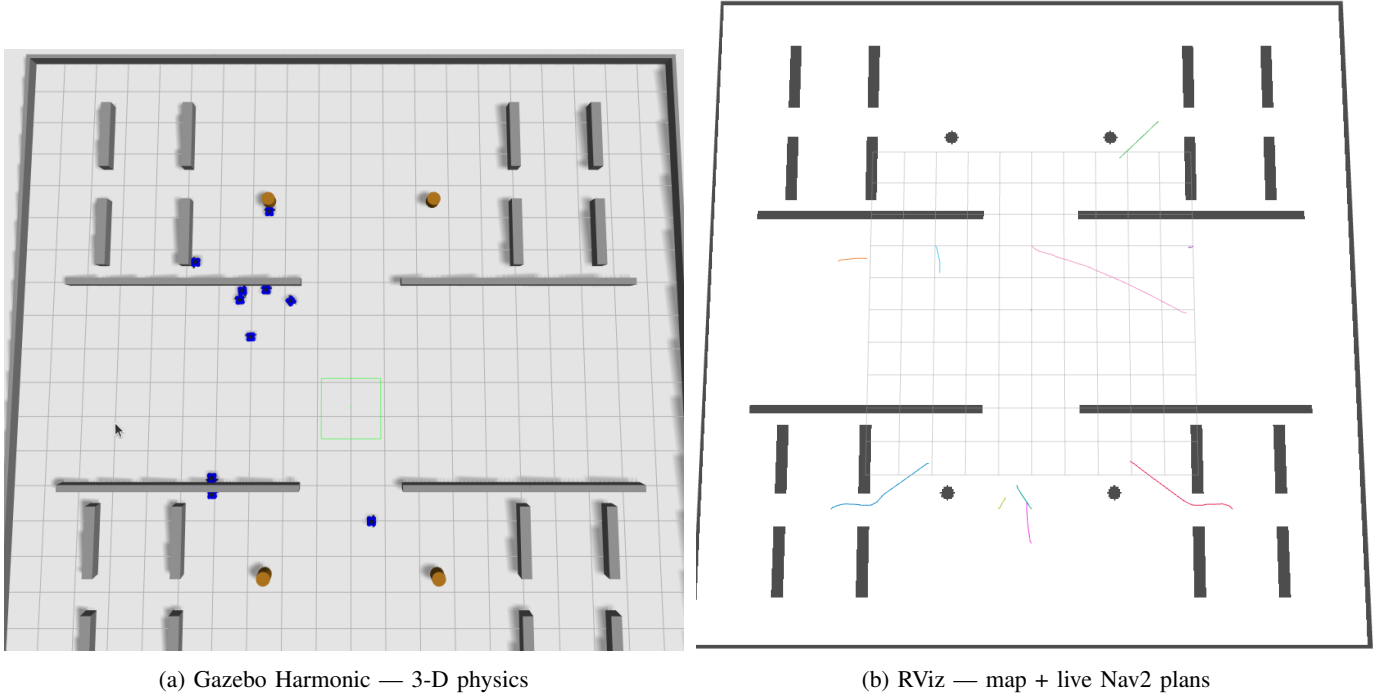
Fig. 7. Representative live snapshot of the largest (10-robot) deployment executing under AHE-MRTA on a dynamic_task_arrival instance. (a) Gazebo Harmonic 3-D physics: the ten TurtleBot3 WafflePi robots (blue) dispersed across the 20×20 m inspection arena—divider walls, square pillars, and cylinder obstacles (orange)—each driving to an assigned inspection waypoint. (b) The concurrent RViz view in the shared map frame: the pre-built occupancy map overlaid with each robot's current Nav2 global plan (one colour per robot) and ground-truth pose. The colour-coded plans show the fleet fanned out across both lanes—the visual signature of the ecosystem's per-event, work-conserving dispatch.
