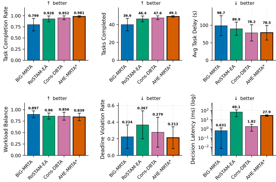
Fig. 9. Multi-metric results at the 10-robot scale (60 runs: four methods, three scenarios, and five seeds; the three scenarios are pooled, so each bar is n=15 ; mean \pm standard deviation; decision latency on a log scale). Pooled over scenarios, AHE-MRTA leads on completion (0.981 versus 0.799–0.952) and is lowest on deadline violation (0.212 versus 0.224–0.367), at 27.9 ms mean decision latency against 0.6–1.8 ms for the commit-once baselines and 69.1 ms for RoSTAM-EA. Pooling hides where the deadline margin actually comes from: it is concentrated in deadline_pressure (DVR 0.220 versus 0.296–0.504), which the text reports per scenario. The n=5 per-scenario cross-method cells are descriptive and do not establish a corrected ranking.
