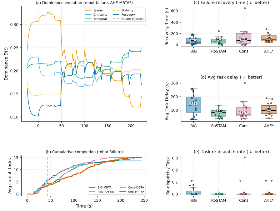
Fig. 11. Interpretable adaptation under robot_failure (3r/15t). Time is measured from each run’s first task activation, so the injection markers in (a) and (b) sit at the scenario’s 45 \pm 5 s offset. (a) Hormone dominance of a representative AHE-MRTA run; the spatial hormone leads the pre-failure phase ( D \approx 0.31 ), and at the injection (dotted line, t \approx 49 s) it collapses while the recovery and stability hormones rise ( 0.12 \rightarrow 0.20 and 0.15 \rightarrow 0.20 ). No single hormone then regains the pre-failure margin: the criticality and temporal channels lead the remainder of the run and the dispatched paradigm alternates between temporal, spatial, and recovery passes. (b) Cumulative task completion (seed-averaged; dotted line: median injection t \approx 44 s): AHE-MRTA continues completing tasks after the failure and reaches the full task set, though it is the last of the three reactive methods to do so. (c–e) Recovery time, average task delay, and task re-dispatch rate as box plots (box: IQR; line: median; whiskers: 1.5 \times \text{IQR} ; points: individual runs, n=15 per method): AHE’s reactivity shows up as the highest recovery-time median (101 s versus 49–77 s); its delay median (98 s) sits between the consensus baselines (72–84 s) and the task-abandoning BiG-MRTA (138 s), and the re-dispatch median is zero for all four methods.
