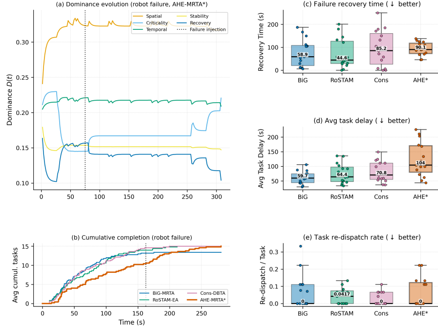
Fig. 10. Interpretable adaptation under robot_failure (3r/15t). (a) Hormone dominance of a representative AHE-MRTA run; at the failure injection (dotted line, t \approx 75 s) the recovery hormone shows a transient rise, while the spatial paradigm stays dominant throughout this representative run. (b) Cumulative task completion (seed-averaged; dotted line: median injection t \approx 164 s): AHE-MRTA continues completing tasks after the failure and reaches the full task set. (c–e) Recovery time, average task delay, and task re-dispatch rate as box plots (box: IQR; line: median; whiskers: 1.5 \times \text{IQR} ; points: individual runs, n=15 per method): AHE’s reactivity costs higher task delay and re-dispatch relative to the commit-once baselines.
